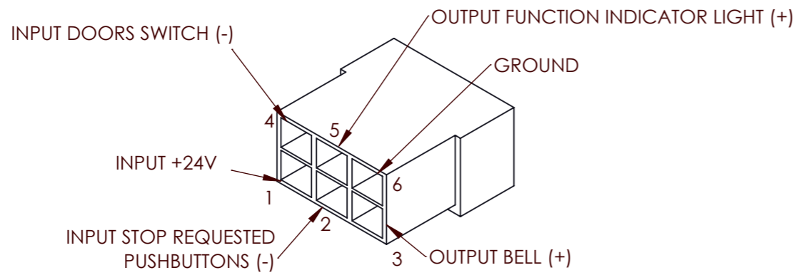
PINOUT ASIGNMENT
